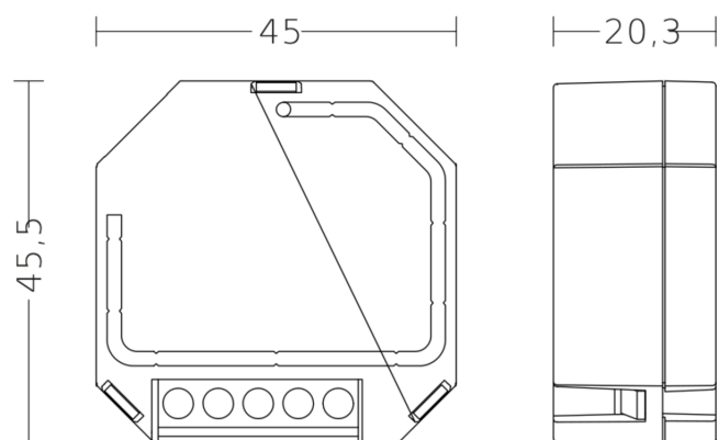
Dimension Drawing
