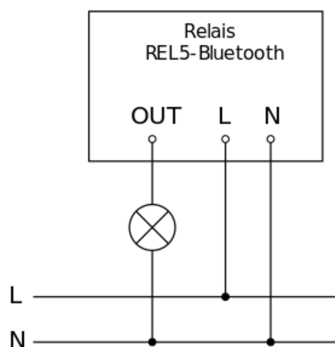
Circuit diagram 1
